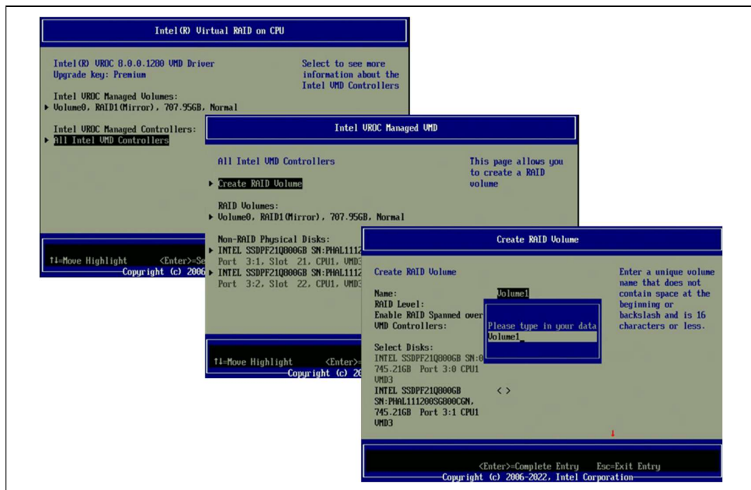
Figure 2-7. Create NVMe RAID Volume Option in BIOS
