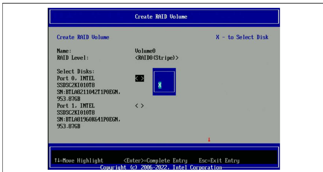
Figure 2-18. Drives Selection for SATA RAID Volume Creation
