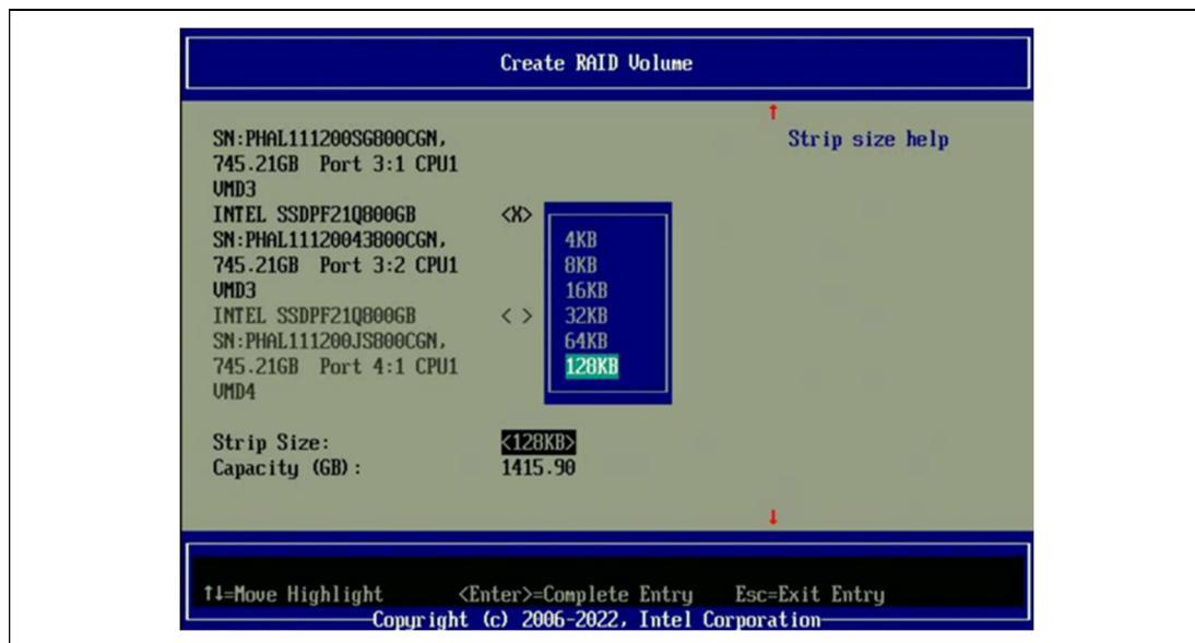
Figure 2-10. Strip Size Selection for NVMe RAID Volume Creation
